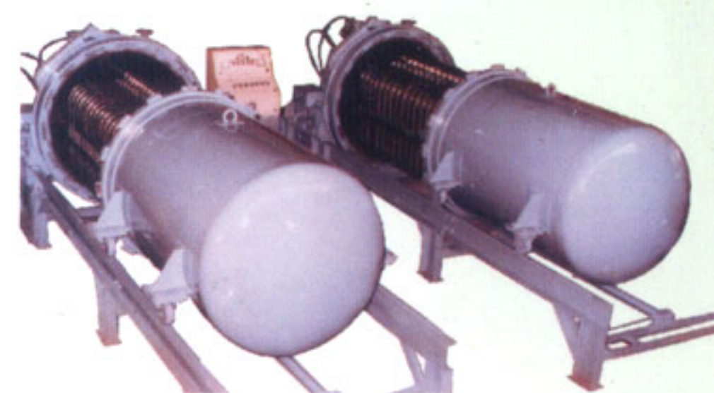
Horizontal pressure leaf filter (shell retraction design) for wax filtration in edible oil plant.
